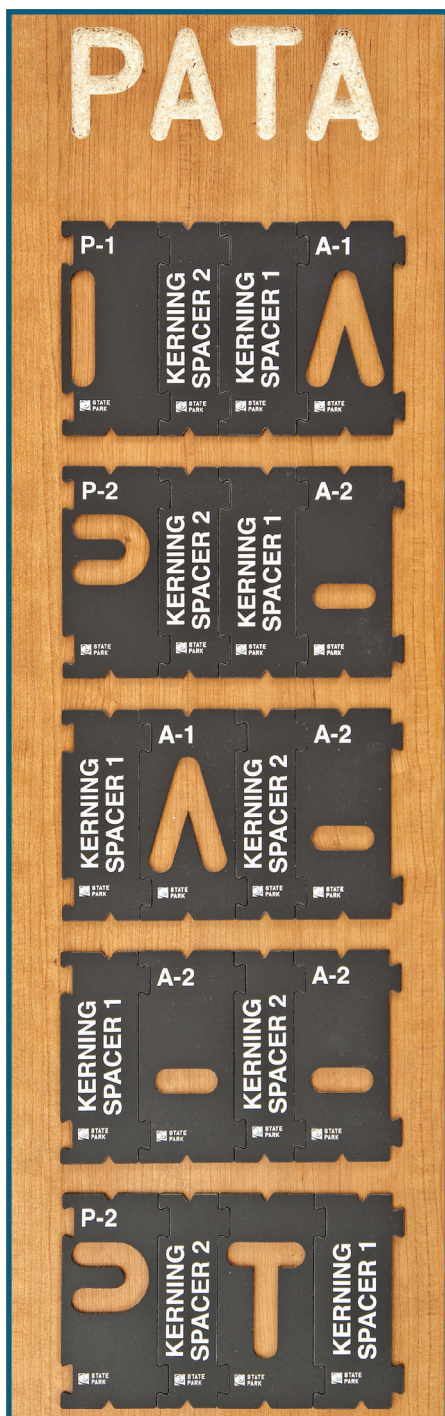
Fig. 7 - Four-Letter Combos
