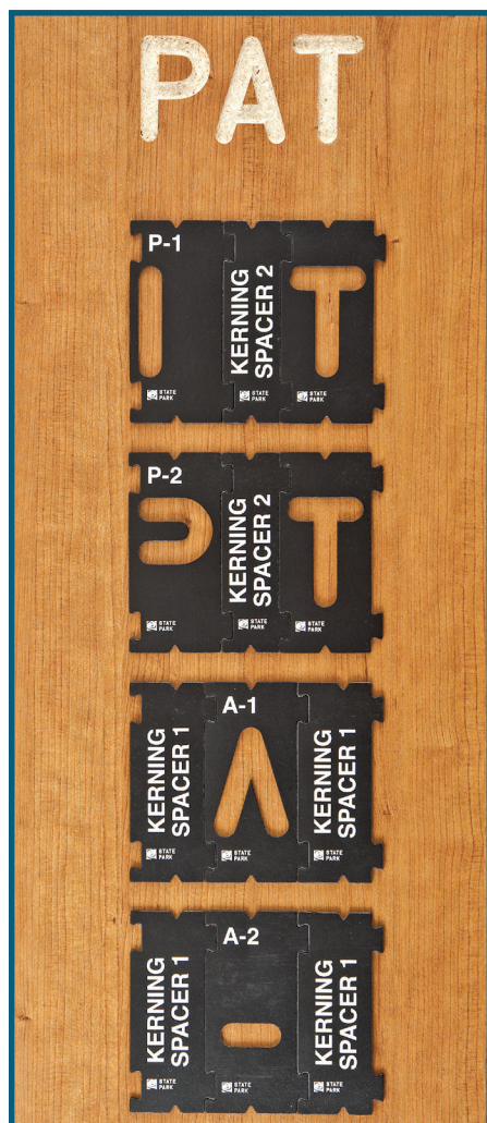
Fig. 6 - Three-Letter Combos
