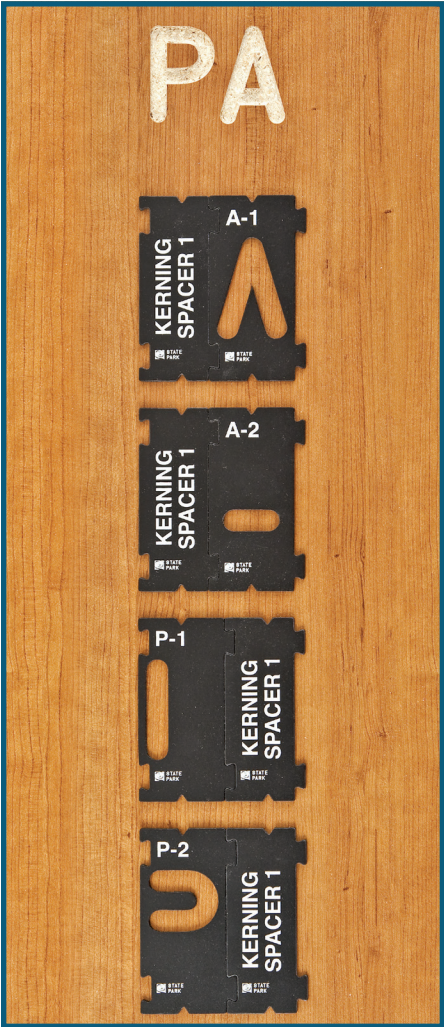
Fig. 5 - Two-Letter Combos
