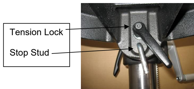
Figure 29: Table Tilt and Tension Lock
