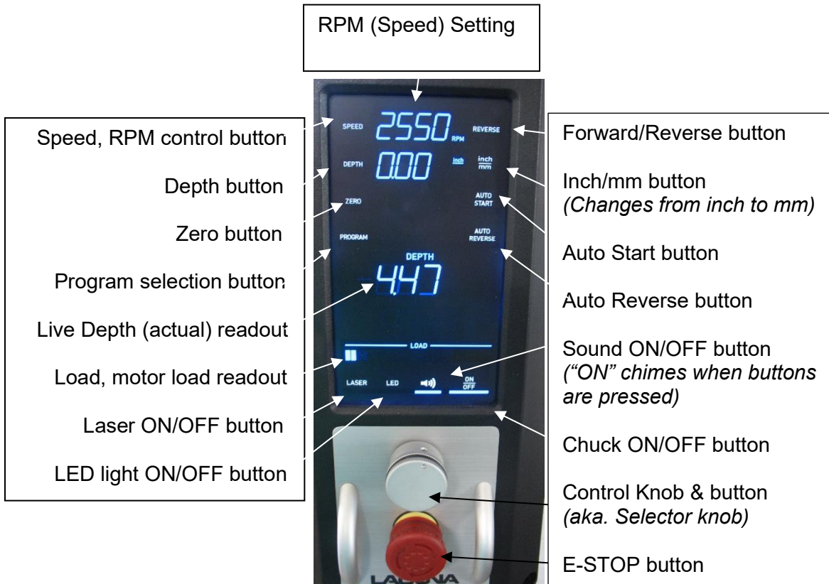
Figure 36: Control Panel
