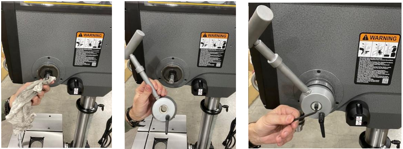
Figures 20-22: Installing handle (right or left side)
