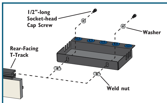
Mounting to a Fence with Rear-Facing T-Track
