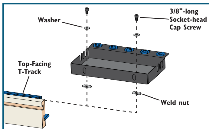
Mounting to a Fence with Top-Facing T-Track
